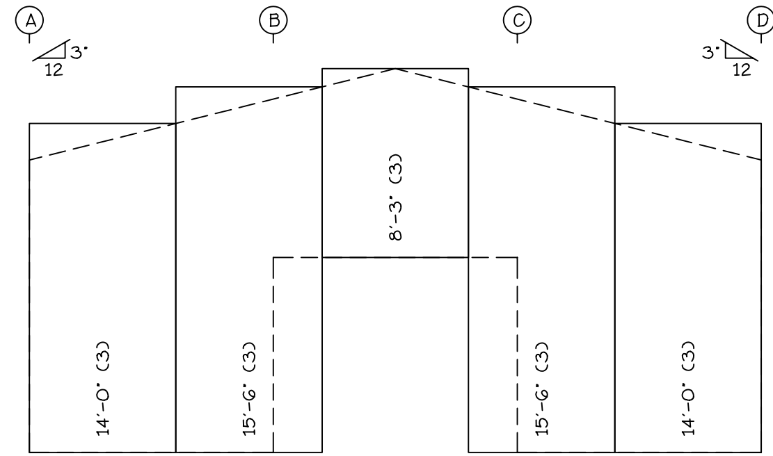
ENDWALL INSULATION: FRAME LINE 1
