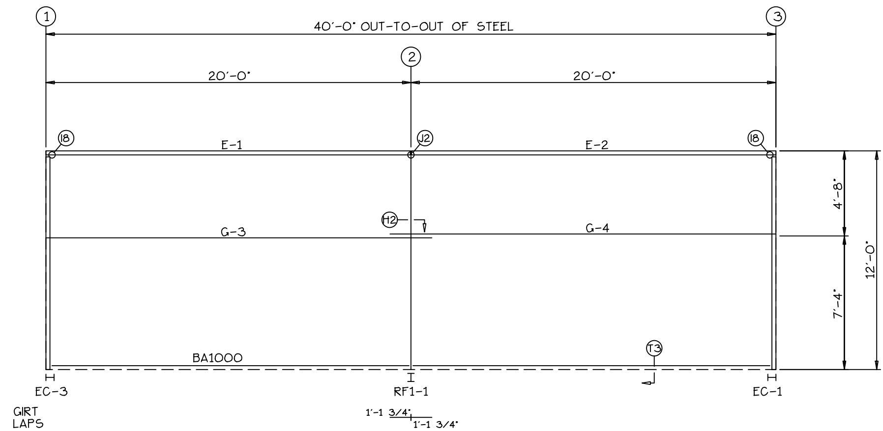
SIDEWALL FRAMING: FRAME LINE D
