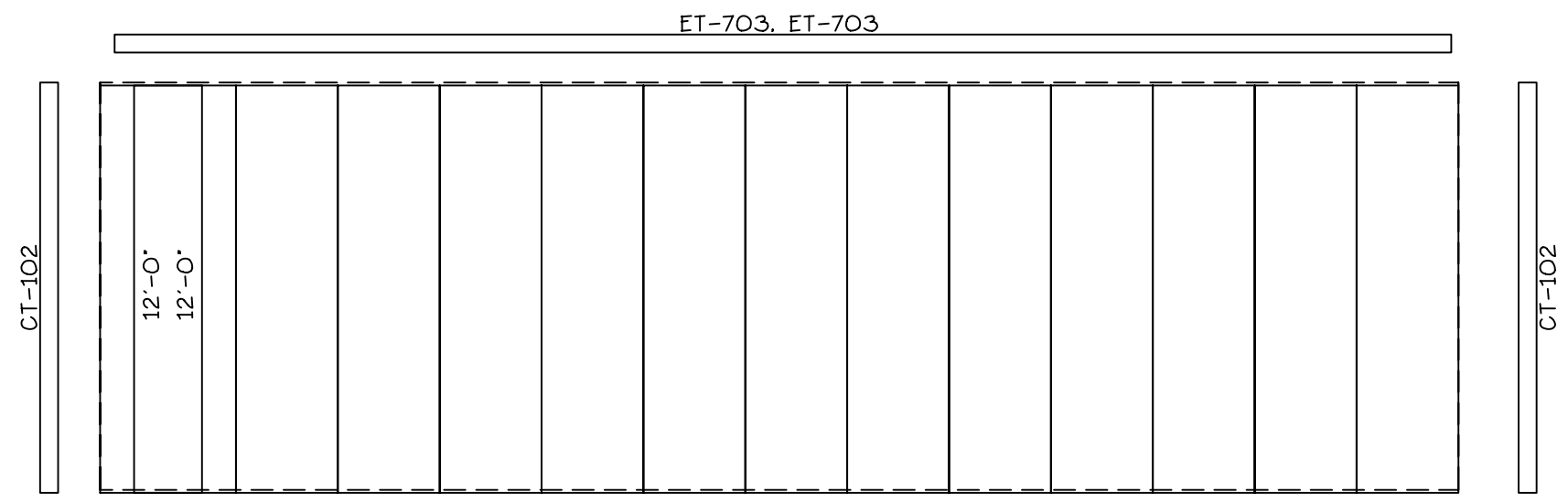
SIDEWALL SHEETING + TRIM: FRAME LINE D PANELS: 26 Ga. PR - NEED COLOR
