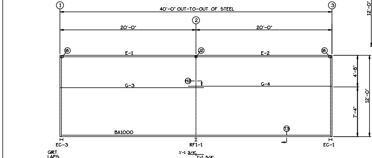
SIDEWALL FRAMING: FRAME LINE D
