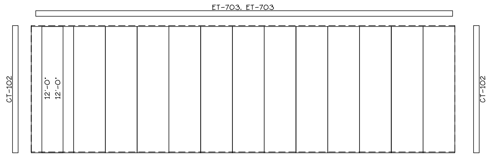
SIDEWALL SHEETING + TRIM: FRAME LINE A PANELS: 26 Ga. PR - NEED COLOR
